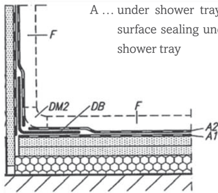
Fig. 11 – Corner formation and sealing in the splash water area. The sealing “F” must be continued behind the tiles. [7.12]
