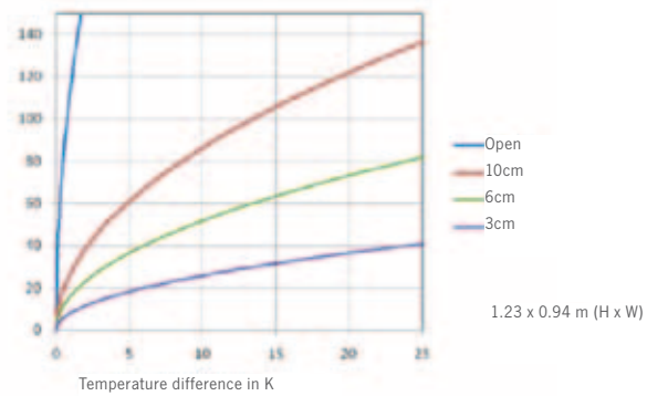
Fig. 8 – Relation of window casement position to the air change rate [7.8]
